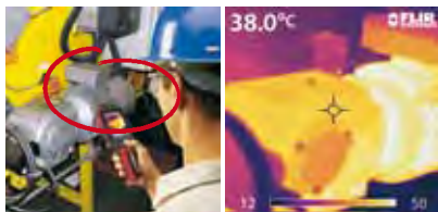
Mechanical check-up of an electrical motor using the FLIR i60.
